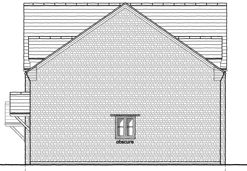
SIDE ELEVATION (PLOT 2)
