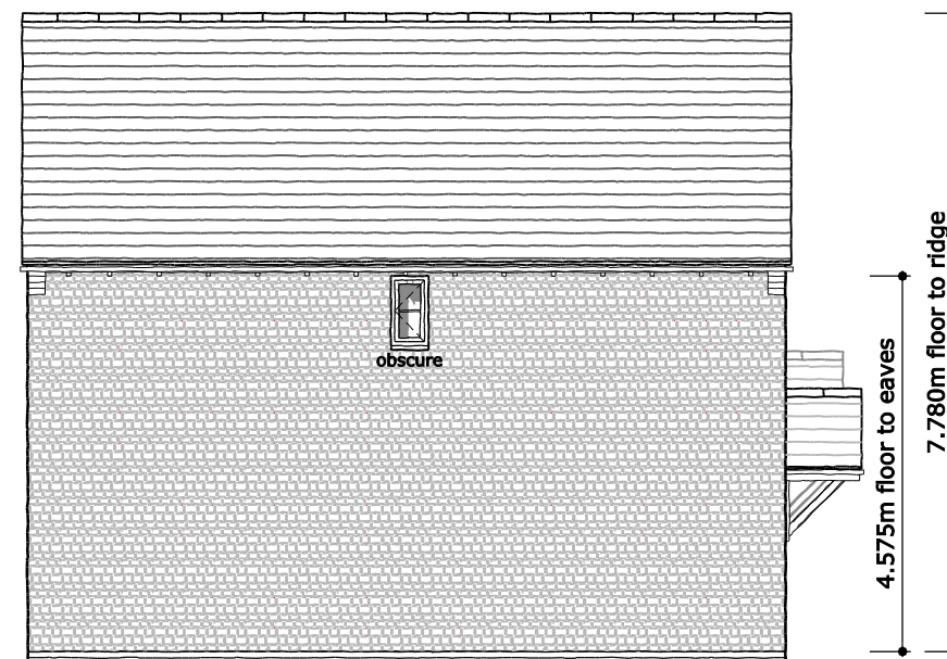
SIDE ELEVATION (PLOT 1)
